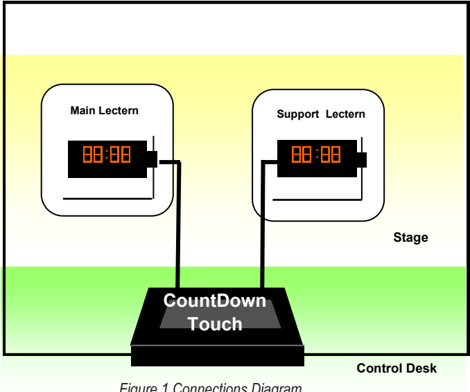
Figure 1 Connections Diagram
